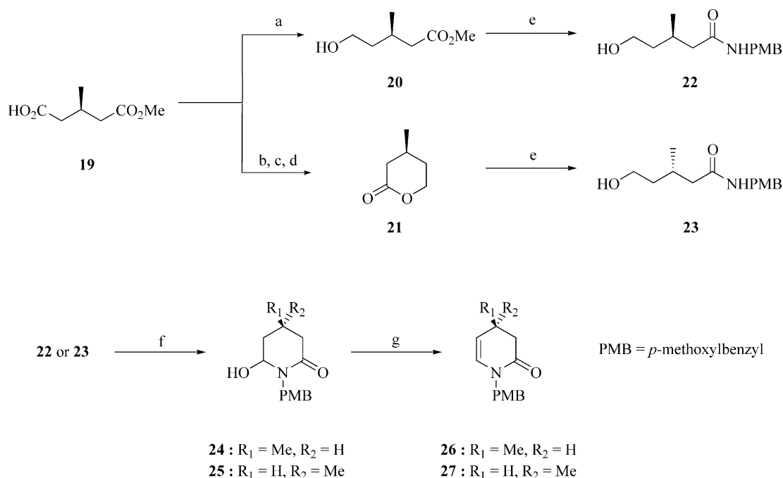
Scheme 1. Synthesis of optically active analogues 26 and 27 . Reagents: (a) \text{BH}_3\cdot\text{SMe}_2 , THF, 0^\circ\text{C} (94%); (b) LiOH aq room temperature; (c) \text{LiBH}_4 , THF, 50^\circ\text{C} ; (d) p\text{-TsOH}\cdot\text{H}_2\text{O} , benzene, reflux (90% in three steps); (e) \text{PMBNH}_2 , toluene, reflux ( 22 : 97%, 23 : 96%); (f) \text{SO}_3\cdot\text{pyridine} , DMSO, \text{Et}_3\text{N} , room temperature ( 24 : 57%, 25 : 43%); (g) p\text{-TsOH}\cdot\text{H}_2\text{O} , toluene, reflux ( 26 : 60%, 27 : 65%).
