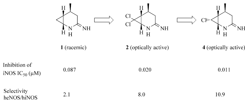
Chart 1. Molecular design of 2-iminopiperidine fused to a substituted cyclopropane.
