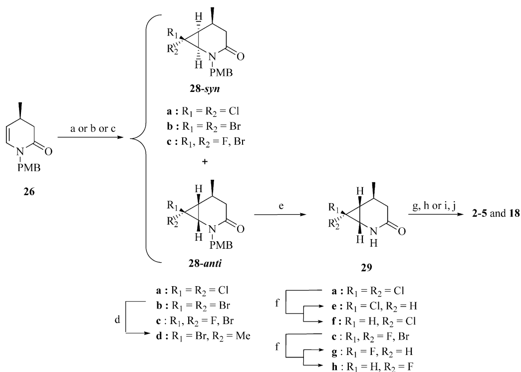
Scheme 2. Synthesis of 2-5 and 18 . Reagents: (a) \text{CHCl}_3 , 50% NaOH aq, aliquat-336 ( 28a-anti : 62%, 28a-syn : 12%); (b) \text{CHBr}_3 , 50% NaOH aq, aliquat-336 ( 28b-anti : 42%, 28b-syn : 12%); (c) \text{FCHBr}_2 , 50% NaOH aq, \text{PhCH}_2\text{NEt}_3\text{Cl} ( 28c-anti : 36%, 28c-syn : 16%); (d) MeI, n -BuLi, THF, -78^\circ\text{C} (91%); (e) \text{BF}_3\cdot\text{OEt}_2 , anisole, 100^\circ\text{C} (75–88%); (f) \text{Ph}_3\text{SnH} , AIBN, benzene, 80^\circ\text{C} ( 29e : 28%, 29f : 53%; 29g : 41%, 29h : 44%); (g) \text{Et}_3\text{O}^+\text{BF}_4^- , \text{CH}_2\text{Cl}_2 ; (h) \text{NH}_3 , EtOH; (i) \text{PhCH}_2\text{NH}_2 , EtOH; (j) 4 M HCl dioxane ( 28-57% in three steps).
