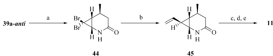
Scheme 7. Synthesis of 11 . Reagents: (a) \text{BF}_3\cdot\text{OEt}_2 , anisole, 100^\circ\text{C} (91%); (b) \text{CuI} , \text{CH}_2=\text{CHMgBr} , \text{Et}_2\text{O} –THF (59%); (c) \text{Et}_3\text{O}^+\text{BF}_4^- , \text{CH}_2\text{Cl}_2 ; (d) \text{NH}_3 , \text{EtOH} ; (e) 4 M \text{HCl} dioxane (6% in three steps).
