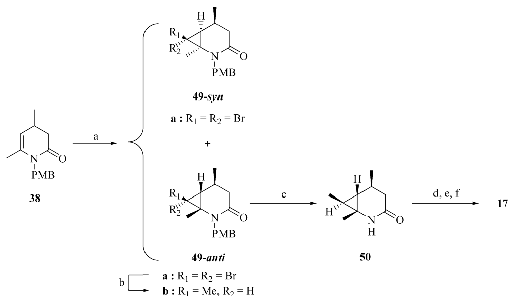
Scheme 9. Synthesis of 17 . Reagents: (a) \text{CHBr}_3 , 50% NaOH aq, aliquat-336 ( 49a-anti : 26%, 49a-syn : 7%); (b) \text{CuSCN} , MeLi, \text{Et}_2\text{O} –HMPA, then \text{NH}_4\text{Cl} aq (65%); (c) \text{BF}_3 \cdot \text{OEt}_2 , anisole, 100^\circ\text{C} (90%); (d) \text{Et}_3\text{O}^+ \text{BF}_4^- , \text{CH}_2\text{Cl}_2 ; (e) \text{NH}_3 , \text{EtOH} ; (f) 4 M HCl dioxane (48% in three steps).
