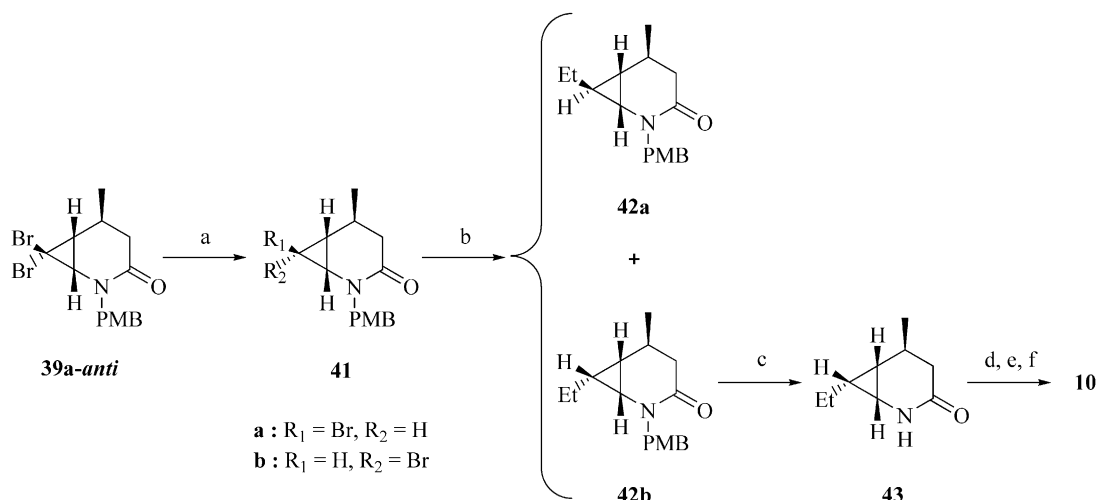
Scheme 6. Synthesis of 10 . Reagents: (a) n\text{-Bu}_3\text{SnH} , toluene, -10^\circ\text{C} (78%, 41a : 41b = 1:3); (b) \text{CuI} , n\text{-BuLi} , THF, then \text{EtI} ( 42a : 20%, 42b : 18%); (c) \text{BF}_3\cdot\text{OEt}_2 , anisole, 100^\circ\text{C} (39%); (d) \text{Et}_3\text{O}^+\text{BF}_4^- , \text{CH}_2\text{Cl}_2 ; (e) \text{NH}_3 , \text{EtOH} ; (f) 4 M \text{HCl} dioxane (88% in three steps).
