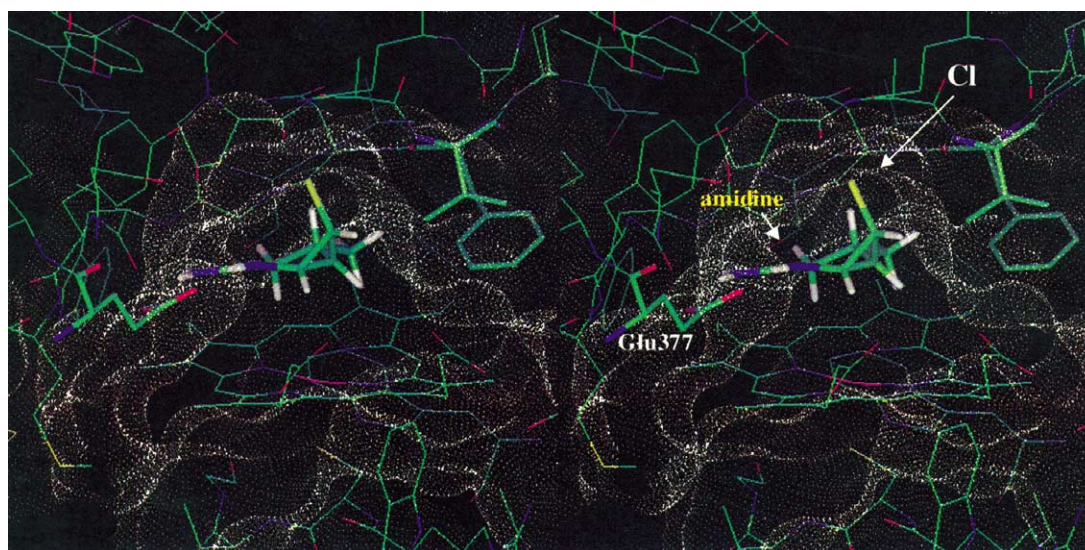
Figure 3. Stereo view of a docking model of compound 4 with human iNOS (PDB code 2NSI).
